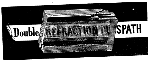
Fig. 17.—Double refraction of Iceland spar.
